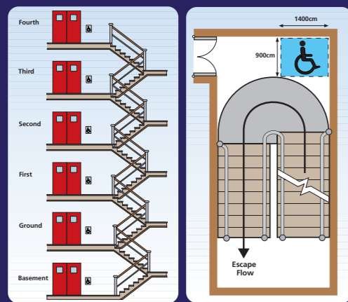
Examples of a Type B outstation installed in the protected stairway providing egress from each storey or stairway or an
